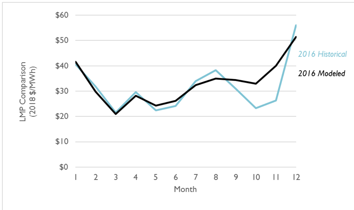
Figure 29. Comparison of 2016 historical and simulated 2016 locational marginal prices for the WCMA region (monthly)
