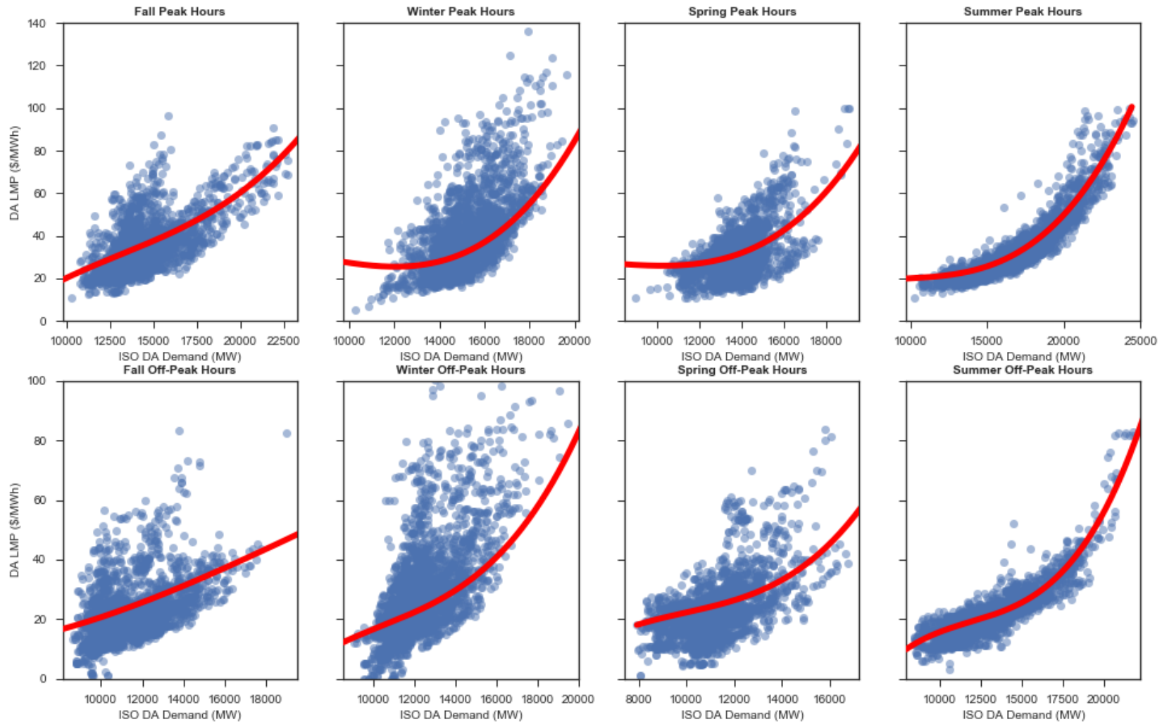
Figure 36. Comparing modeled electricity prices to historical (ISO New England, by season and period, 9/2015–8/2017)
