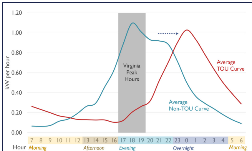
Figure 3. Typical non-TOU EV charging curve versus the California TOU average EV charging curve, with Virginia peak hours
