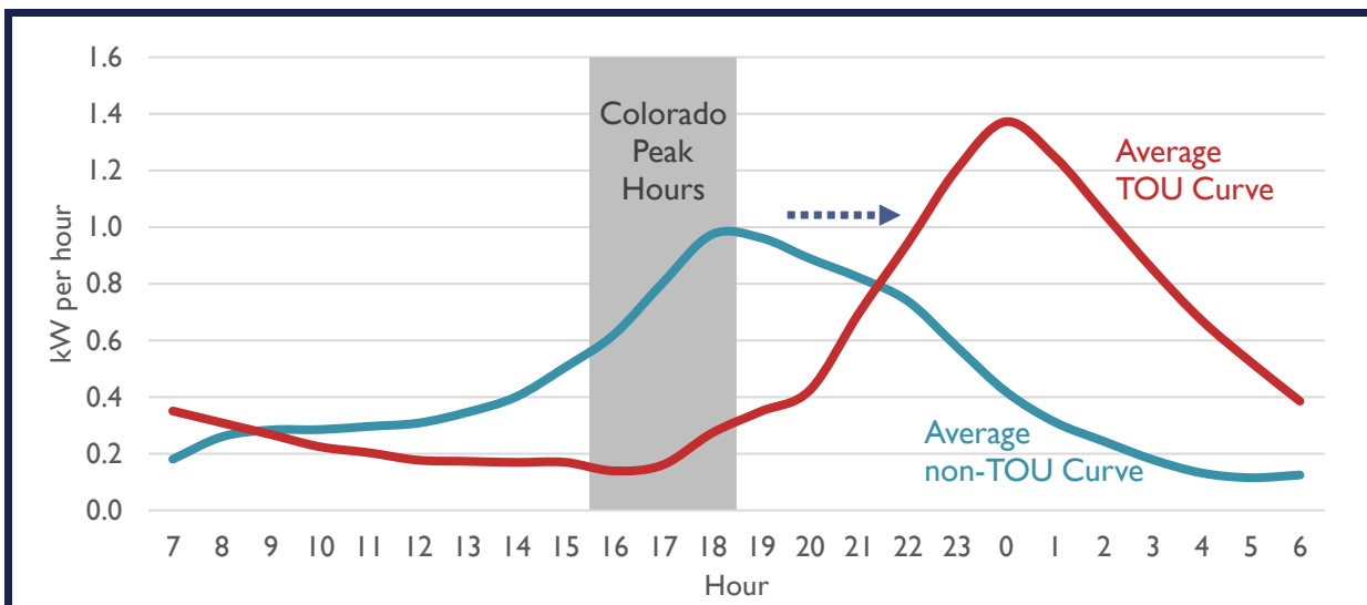
Figure 2. Typical EV charging curve versus the California TOU average EV charging curve, with Colorado peak hours
