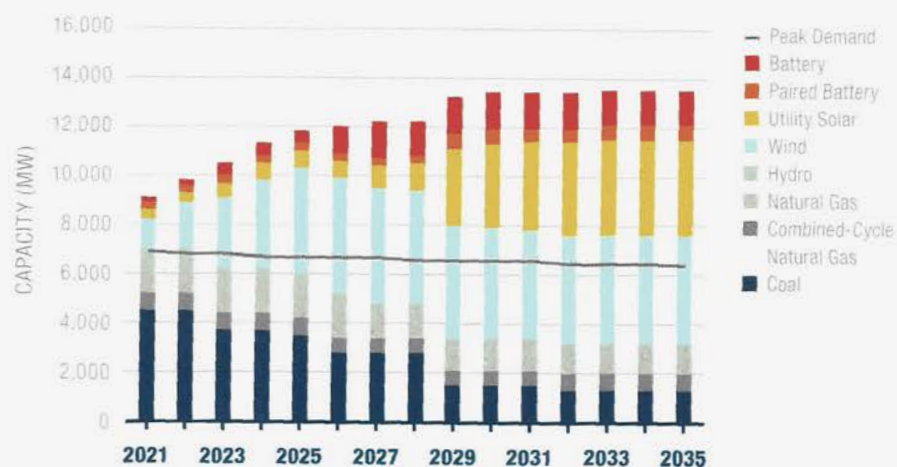
FIGURE 2. APCO NAMEPLATE CAPACITY, RAMPED UP RENEWABLES
