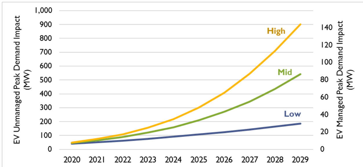
Figure 12. Total New England EV summer peak demand impact with unmanaged and managed charging
