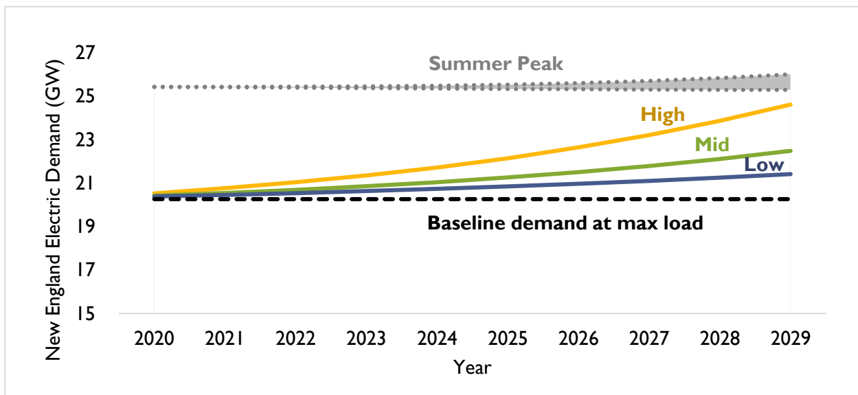
Figure 24. Estimated demand during cold snap’s maximum load hour
